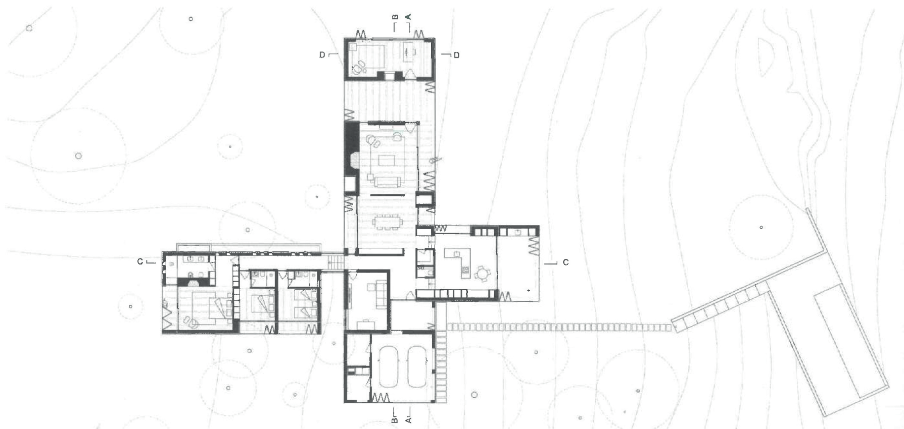
Planta / Floor plan
