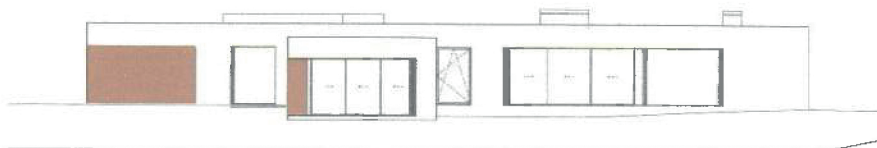
Alzado norte / North elevation
